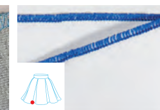
Three Threads Condense Seaming C5-3-32R2/223
